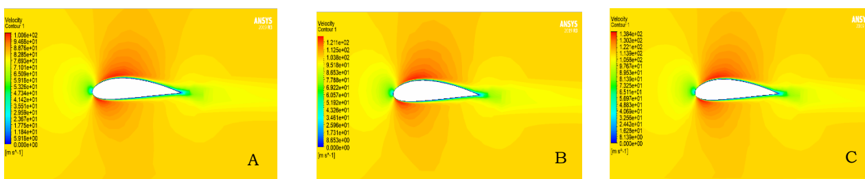
Figure 2. Airfoil a flow pattern with velocity 80, 100, 110 m/s
