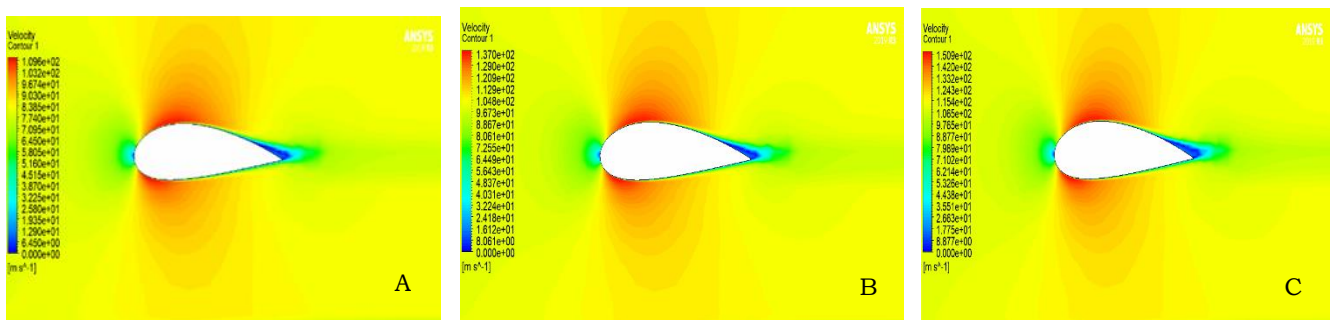
Figure 4. Airfoil c flow pattern with speed 80,100, 110 m/s
